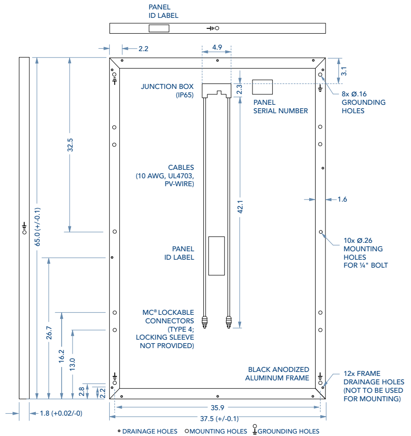
ALL DIMENSIONS IN INCHES; PANEL WEIGHT 41 LBS (18.6 KG)
